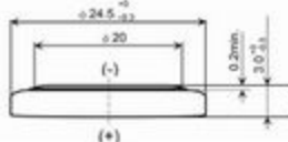
Dimension Drawing
